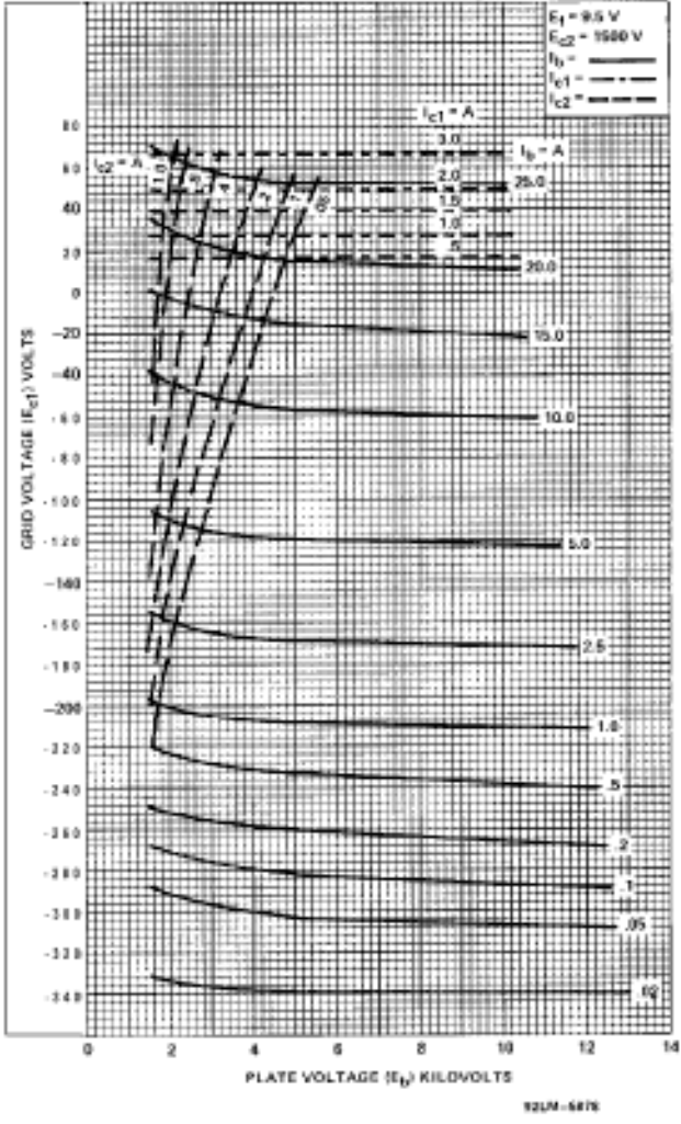
Figure 5- Typical Constant Current Tube Characteristics @ E_{c2} = 1500 V
